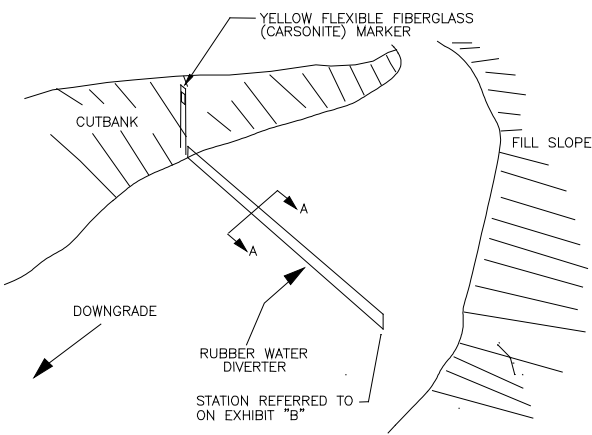
INSTALLATION DETAIL
