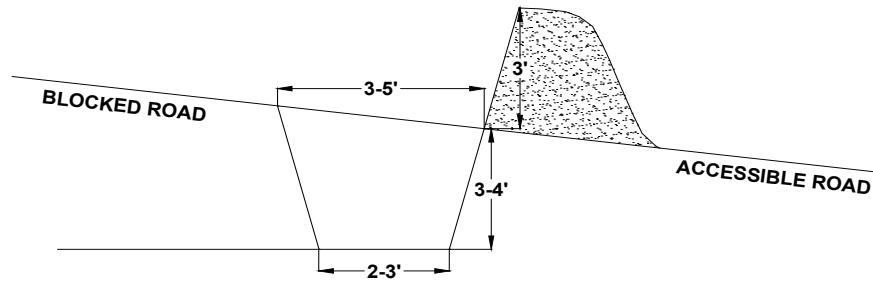
CROSS SECTION
