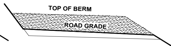
OUTSLOPED
