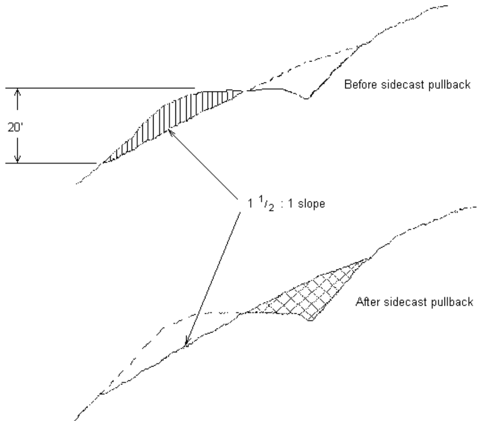
TYPICAL CROSS SECTION VIEW OF SIDECAST PULLBACK AND ROAD REALIGNMENT
