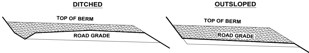
CROSS SECTION
