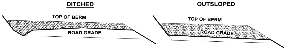
CROSS SECTION
