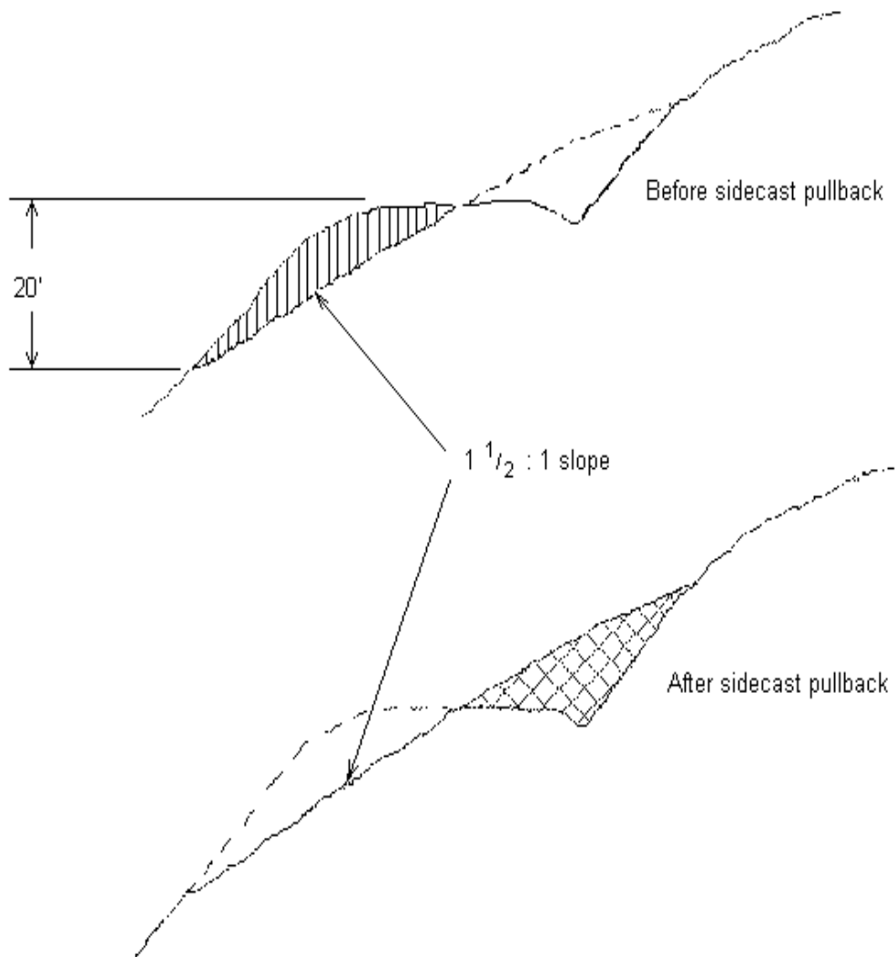
TYPICAL CROSS SECTION VIEW OF ROAD VACATING SIDECAST PULLBACK
