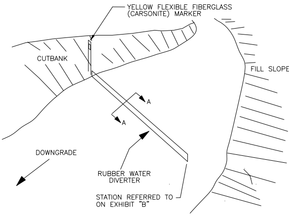
INSTALLATION DETAIL
