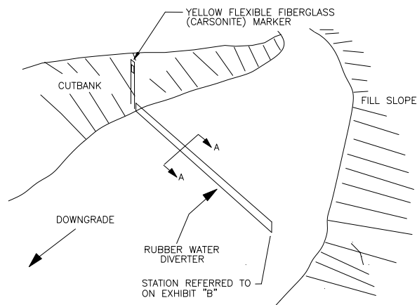
INSTALLATION DETAIL
