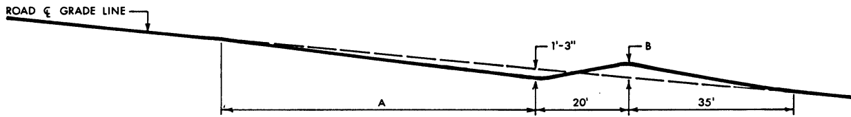
PROFILE (1" = 20')
