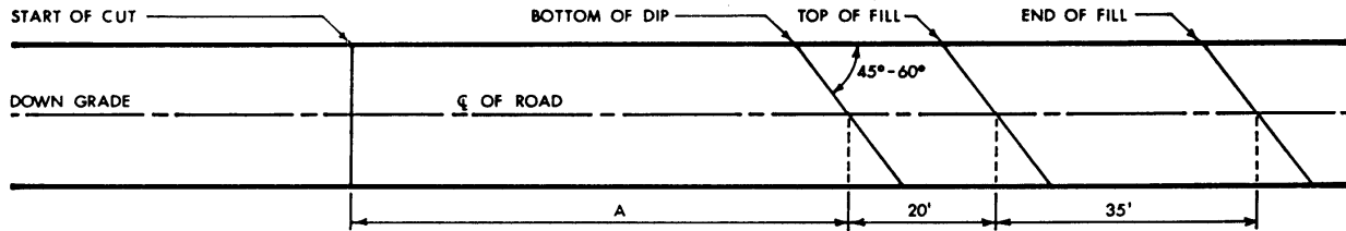
PLAN (1" = 20')
