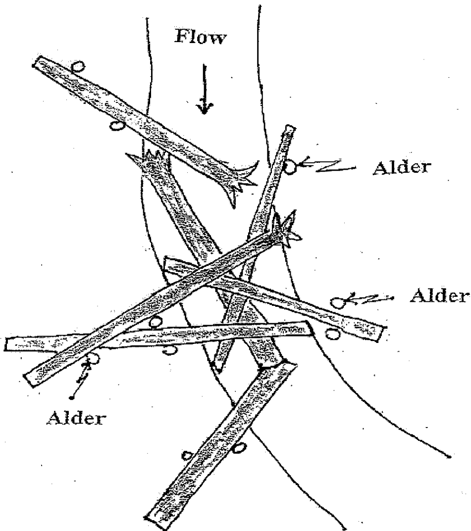
LOG PLACEMENT DIAGRAM (SE2, SE3 – SE6)
