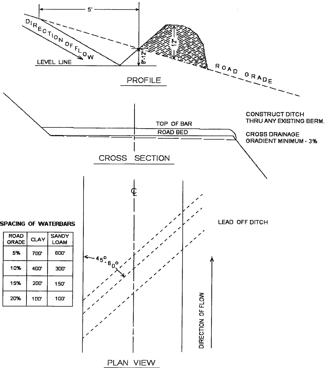
WATERBAR SPECIFICATIONS FOR CROSS DITCHING
