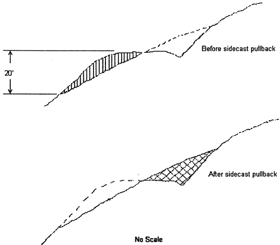
TYPICAL CROSS SECTION VIEW OF ROAD VACATING SIDECAST PULLBACK
